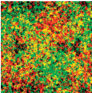
Rot-Grün-Noise
