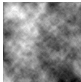
Perlin-Noise
